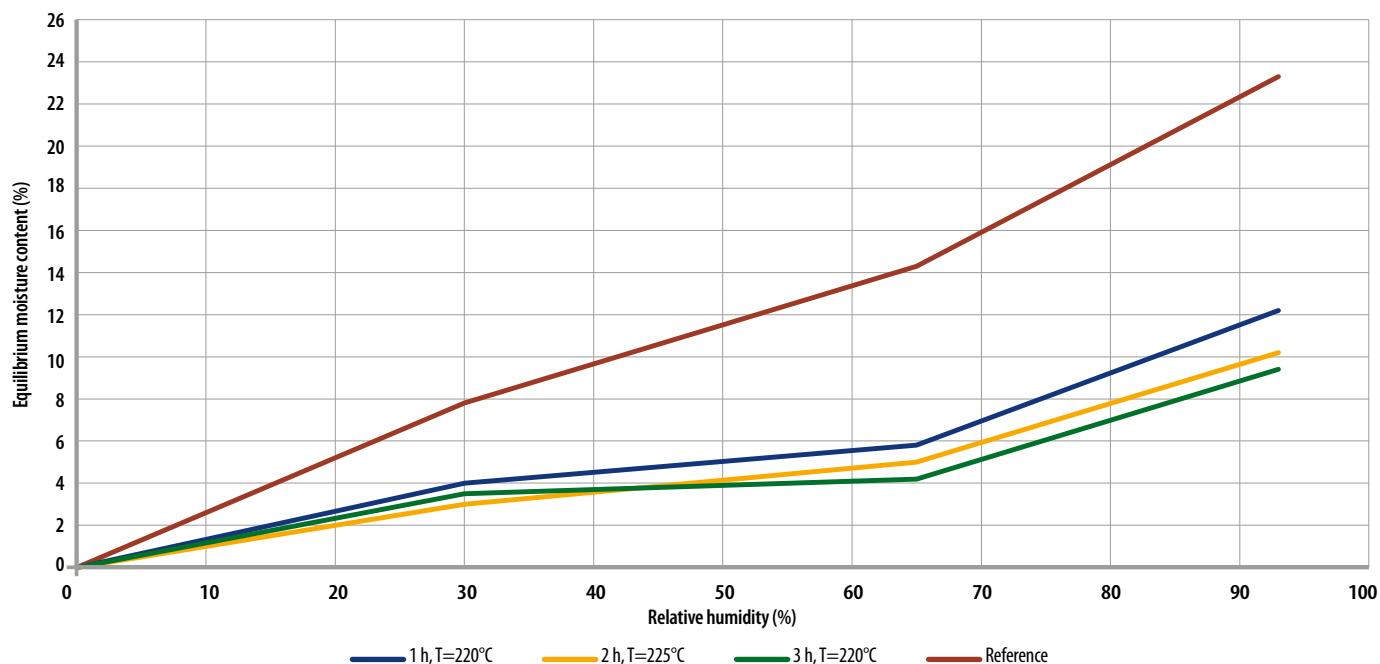
Figure 25. The impact of relative humidity on the equilibrium moisture content of thermally modified spruce (source: VTT).
