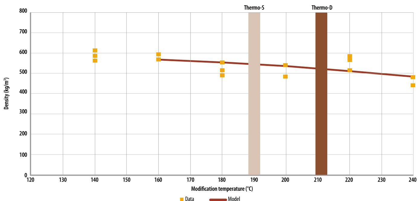
Figure 20. The impact of the modification temperature on the density of ThermoWood® (source: VTT).
