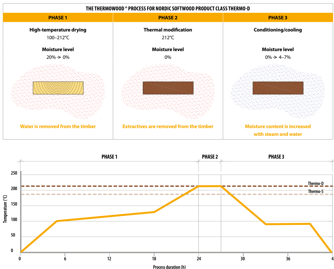
Figure 3. An example of the ThermoWood® process for Nordic softwood (product class Thermo-D).
