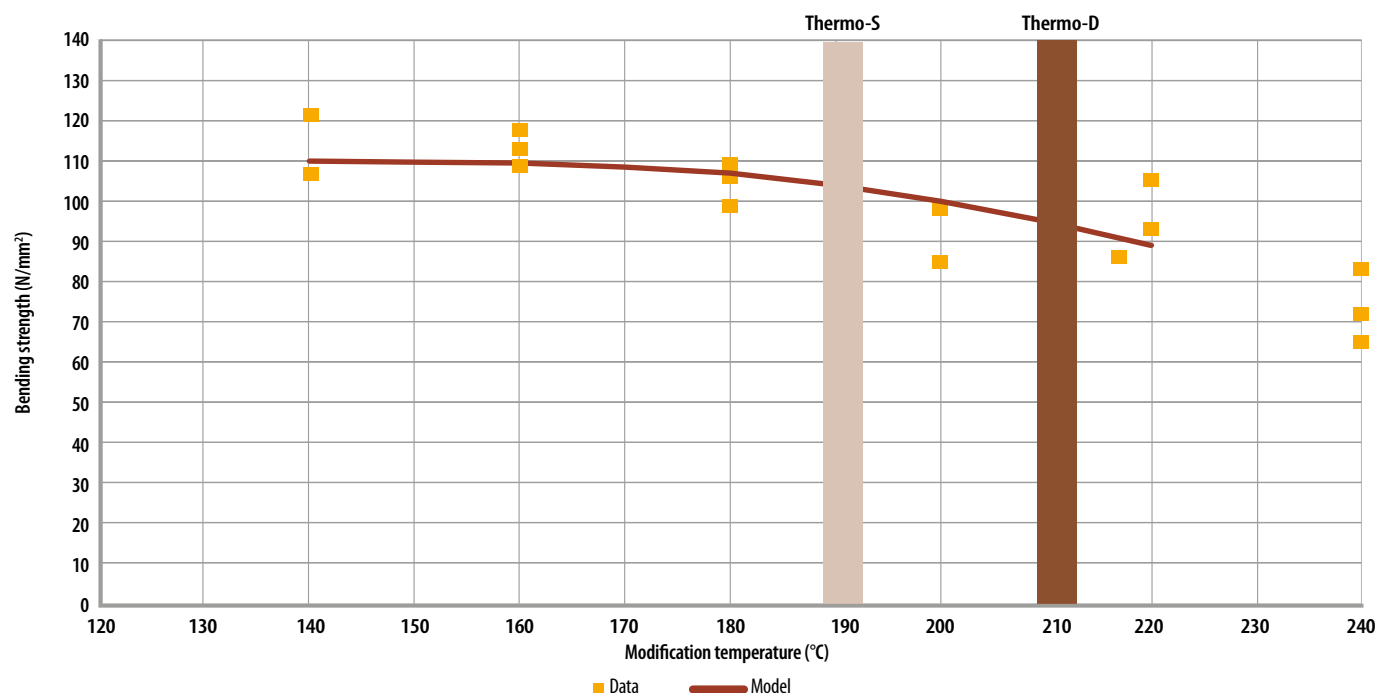
Figure 21. The impact of the modification temperature on the bending strength of ThermoWood® (source: VTT).
