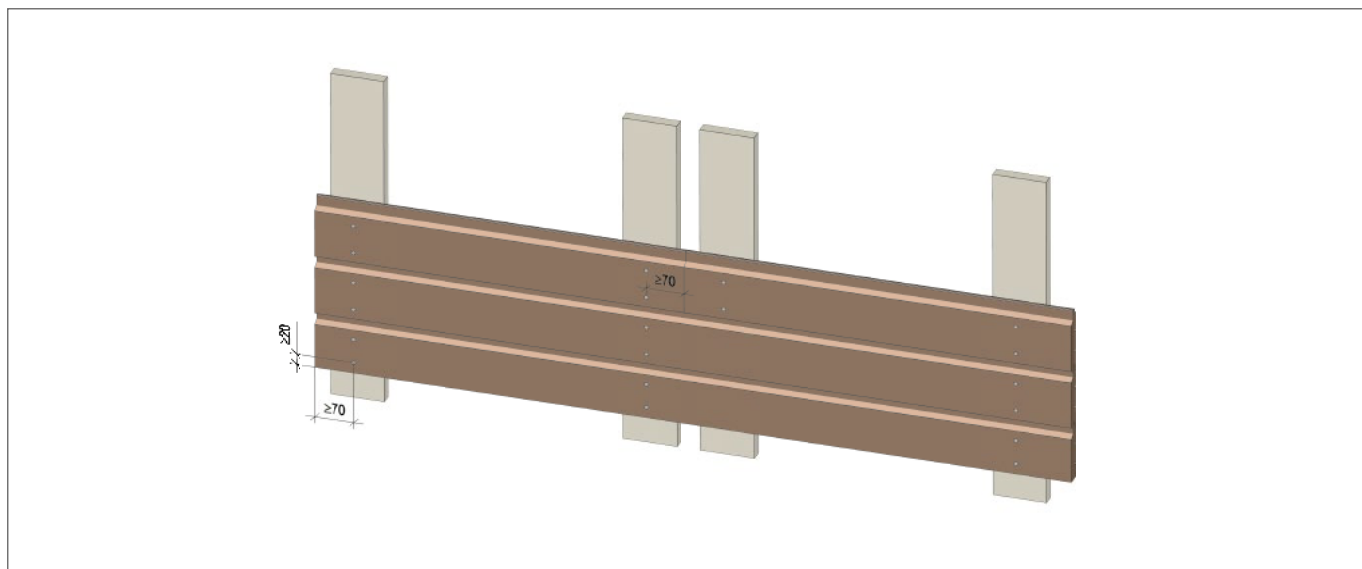
Figure 52. The recommended distances to edges and ends without pre-drilling with ThermoWood® products (without tongue and groove joint).
