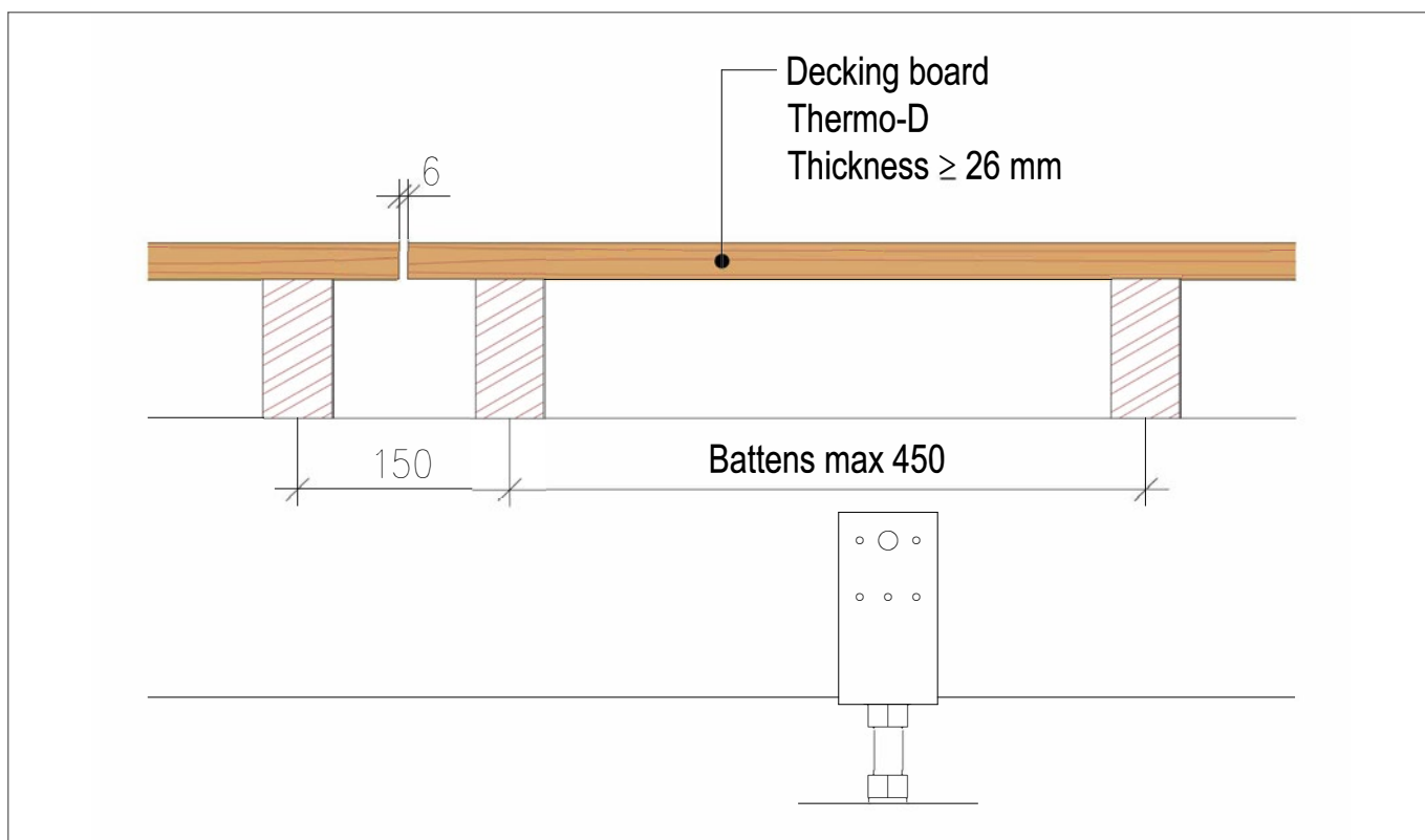
Figure 48. Decking board joint.
