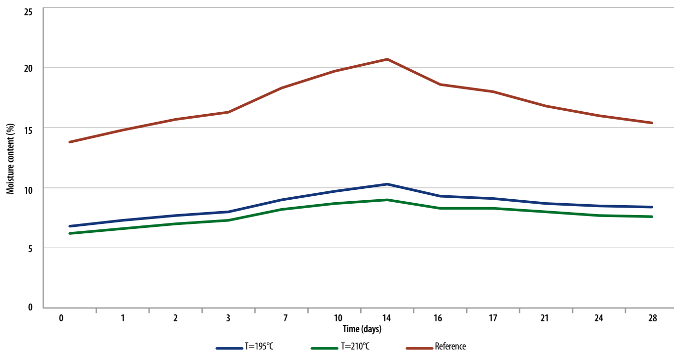
Figure 29. The impact of thermal modification on steam permeability Spruce (source: VTT)
