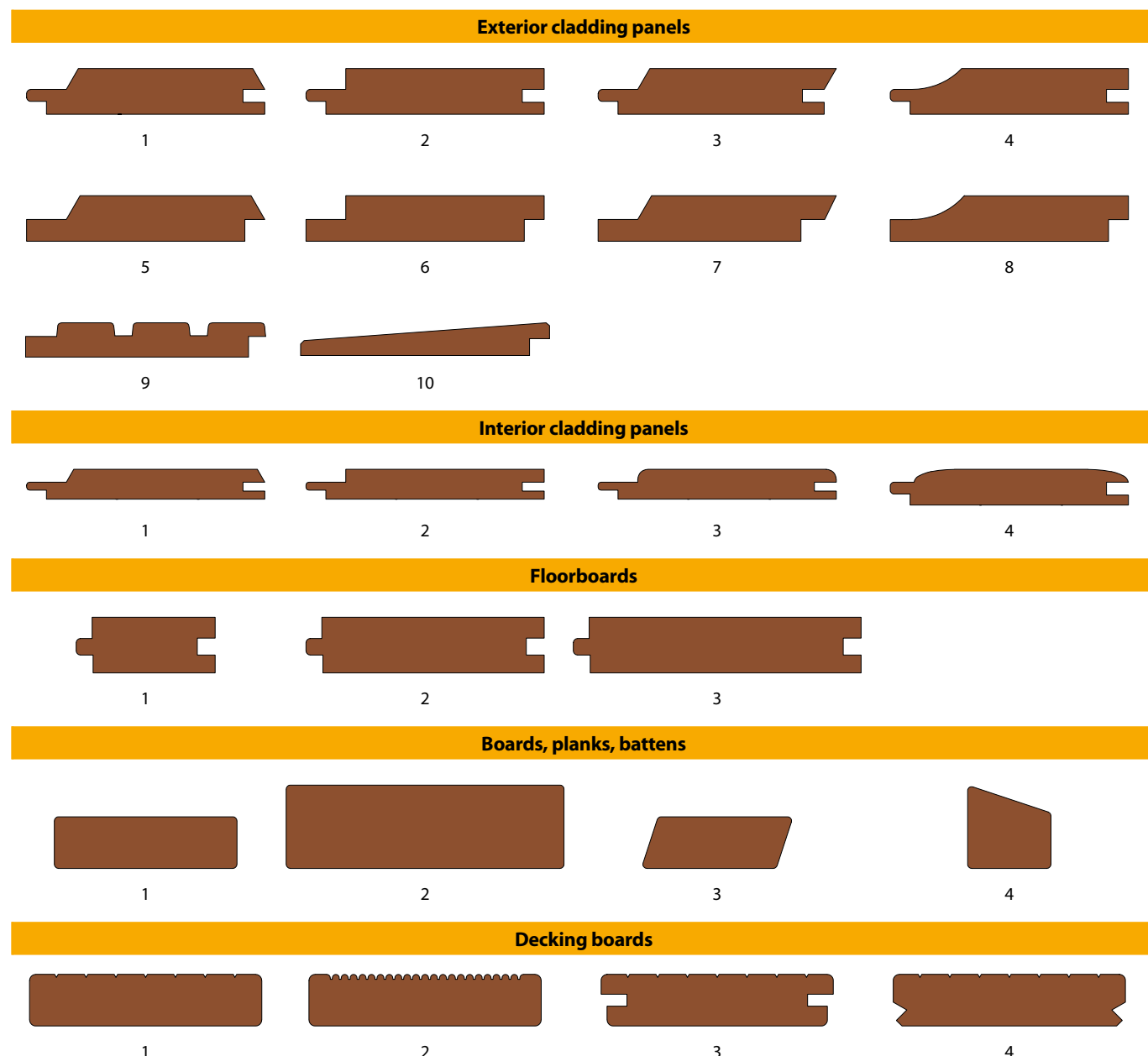
Figure 12. Examples of ThermoWood® profile products.
