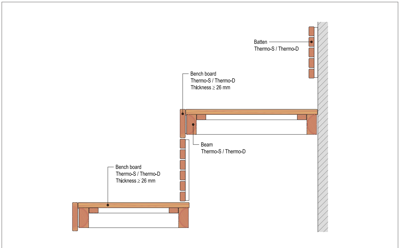
Figure 42. An example of a sauna's bench structures.
