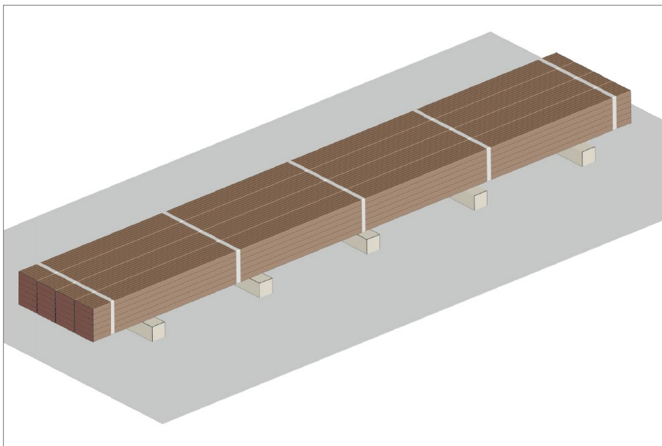
Figure 33. An even surface and a sufficient number of base battens prevent the products from warping.
