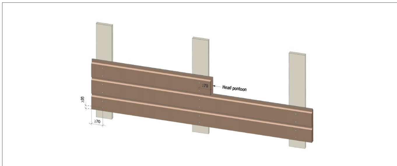
Figure 51. The recommended distances to edges and ends without pre-drilling with ThermoWood® products.
