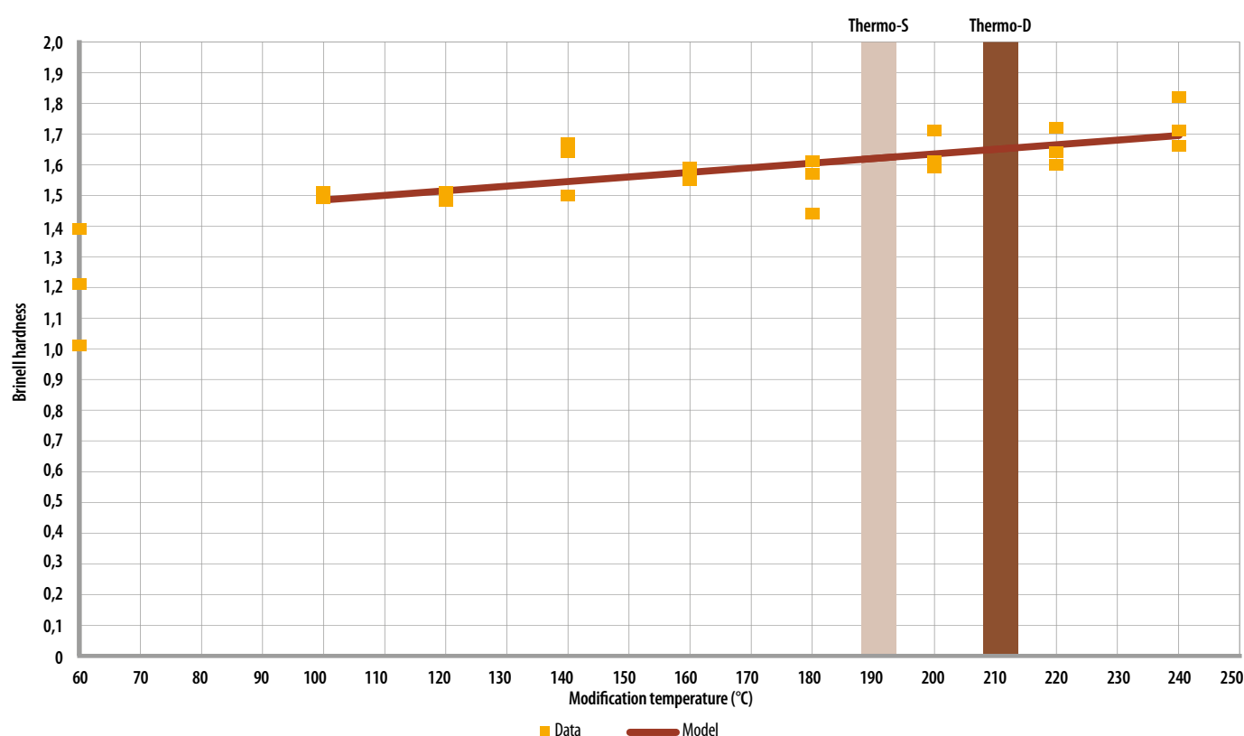
Figure 24. The impact of thermal modification (3 h) on Brinell hardness of pine (source: VTT).
