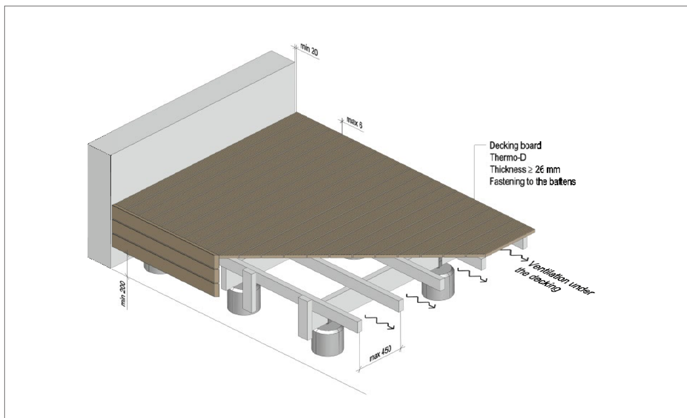
Figure 47. An example of patio structures.
