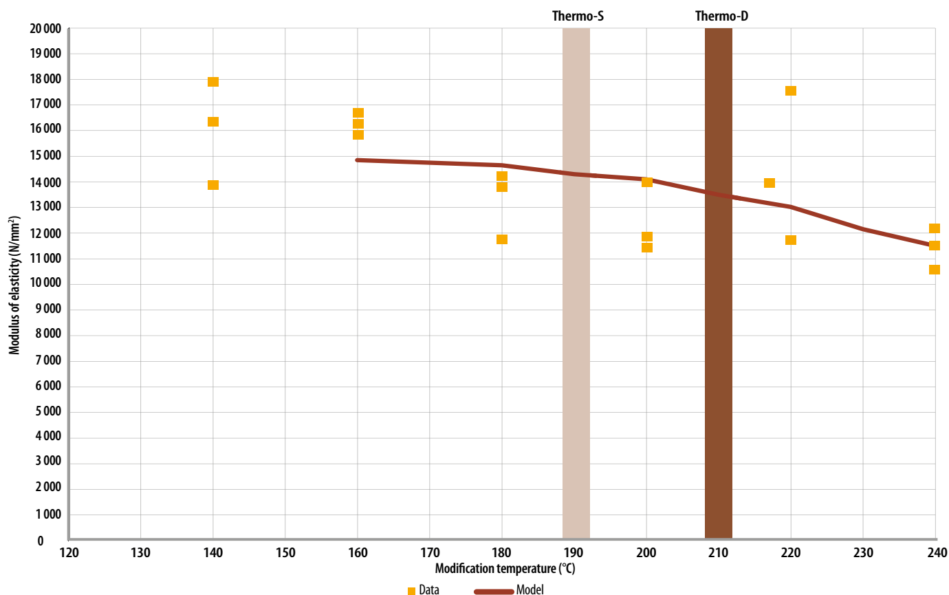
Figure 22. The impact of the modification temperature on the modulus of elasticity of ThermoWood® (source: VTT).
