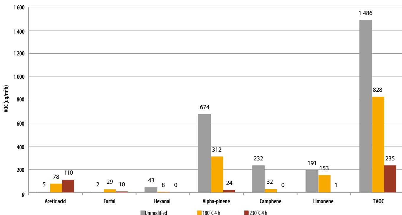
Figure 30. Volatile organic compounds emitted by pine samples after two months (source: VTT).
