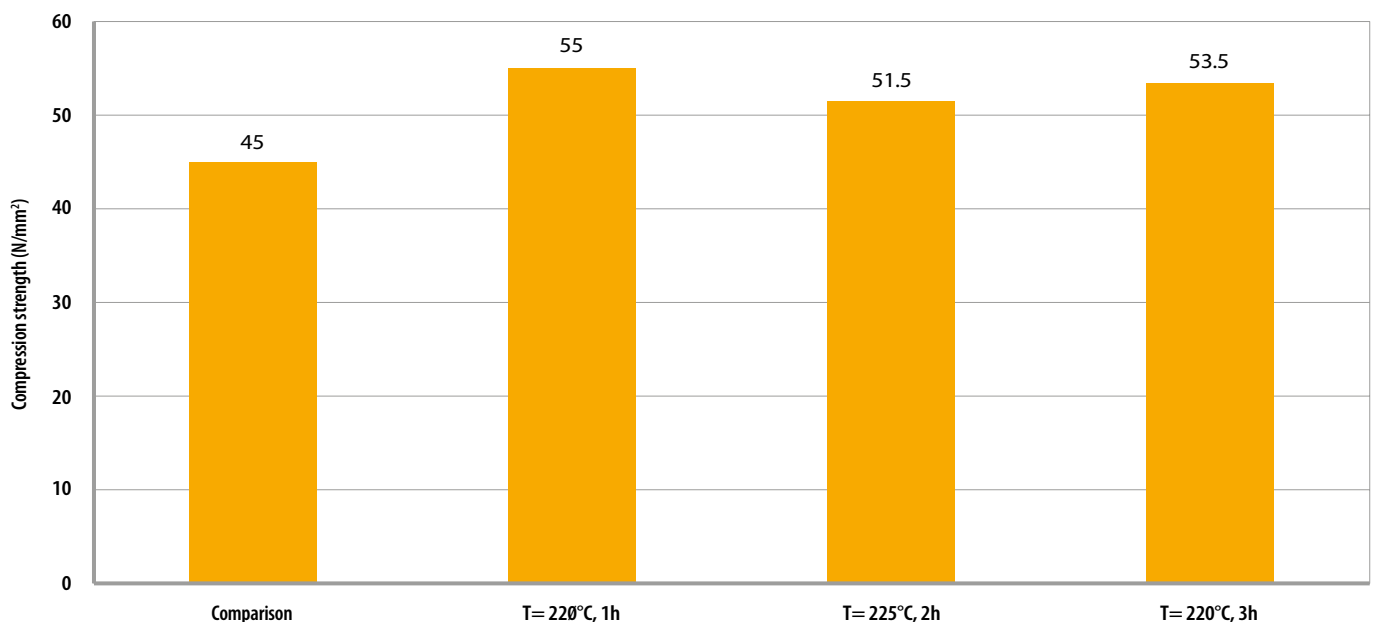
Figure 23. Compression strength parallel to the grain of thermally modified spruce (average density 420 kg/m 3 ) (source: VTT).
