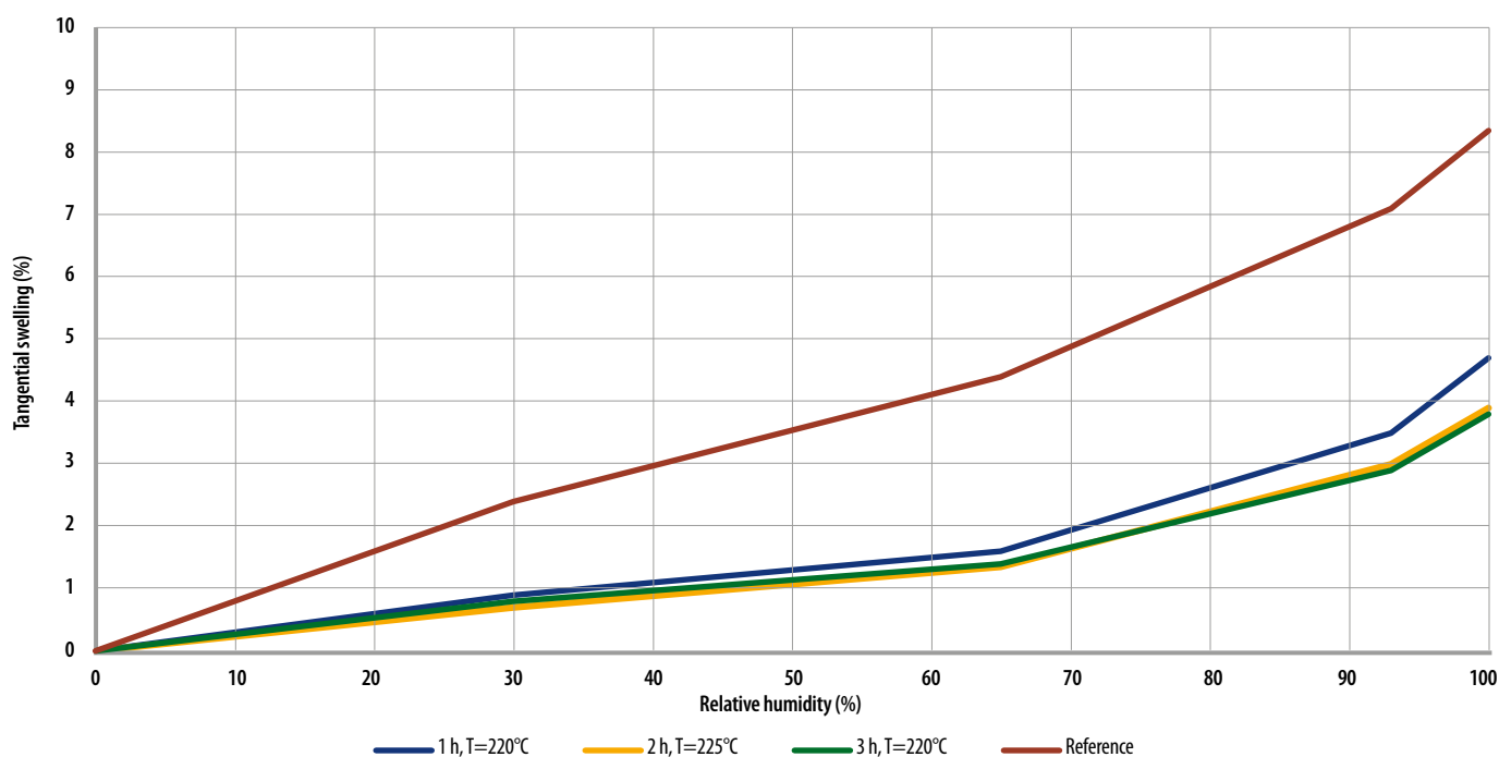
Figure 28. Tangential swelling of spruce as a function of relative humidity (source: VTT).
