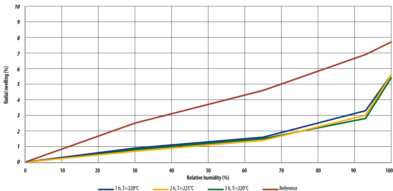
Figure 27. Radial swelling of spruce as a function of relative humidity (source: VTT).
