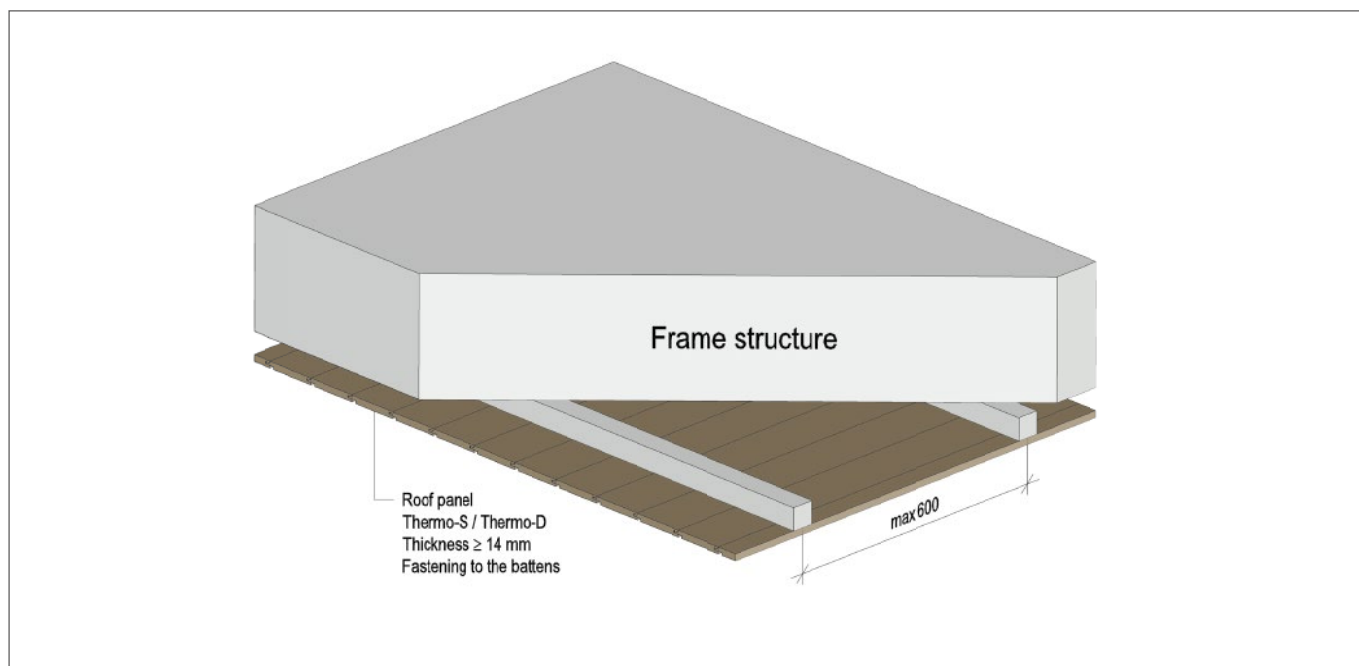
Figure 36. An example of ceiling cladding in a dry space.
