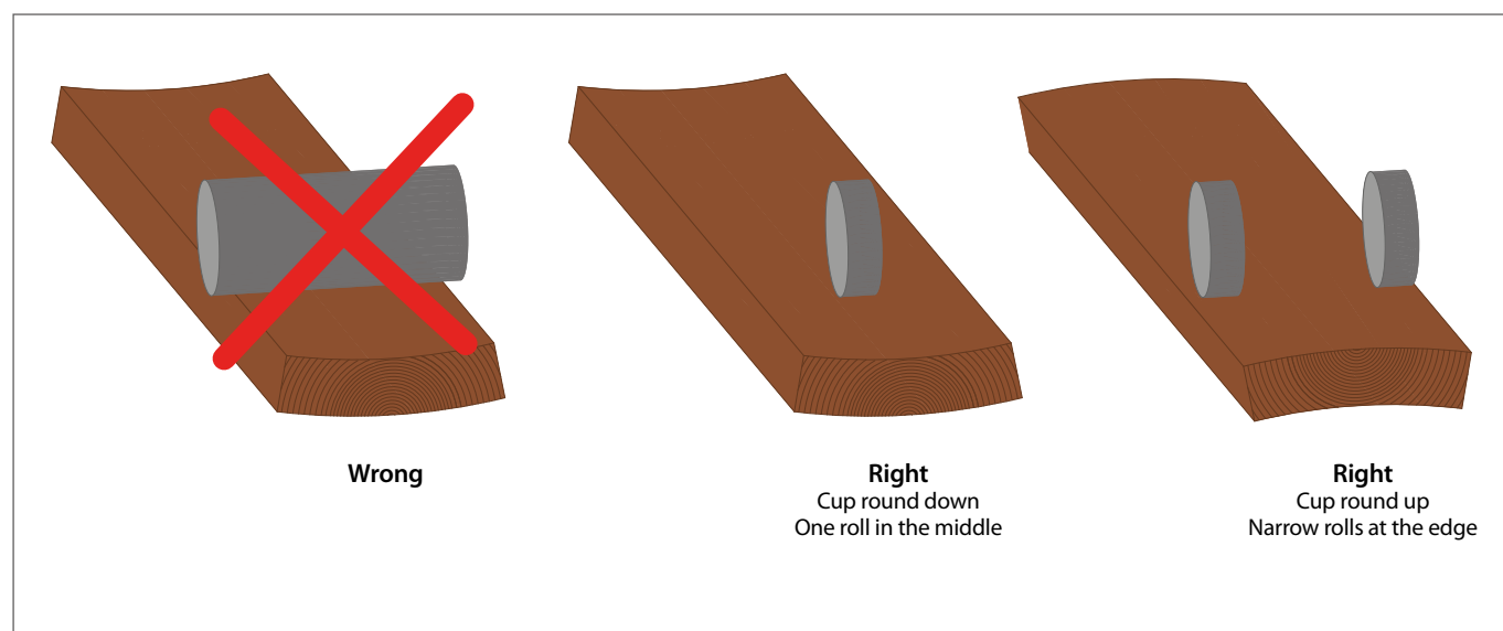
Figure 31. Narrow plane infeed rollers must be used with ThermoWood® products.
