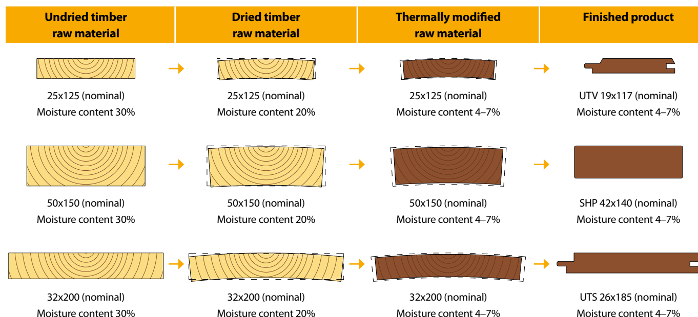
Figure 11. Examples of the impact of thermal modification on product dimensions.
